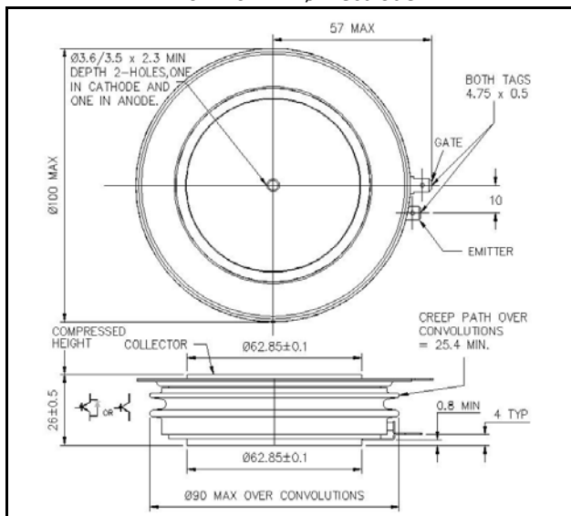
W67 – 62mm \varnothing Electrode
