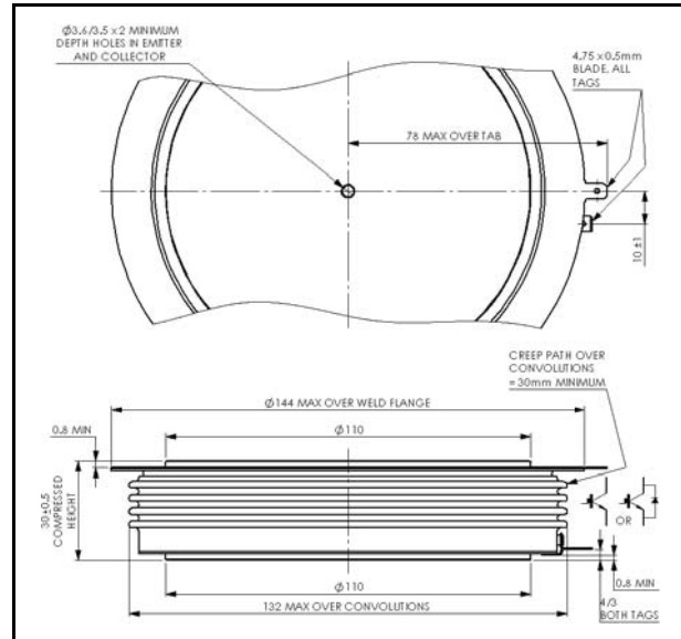
W103 - 132mm \varnothing Electrode
