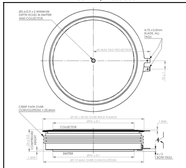
W71 – 96mm \varnothing Electrode
