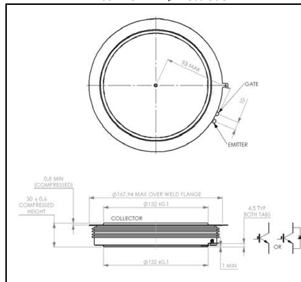
W110 - 132mm \varnothing Electrode
