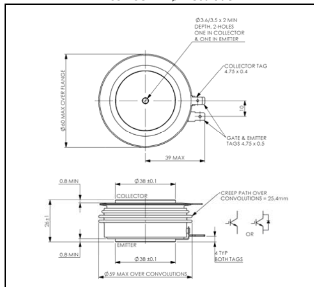
W109 - 38mm \varnothing Electrode
