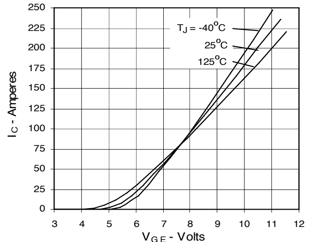
Fig. 6. Input Admittance
