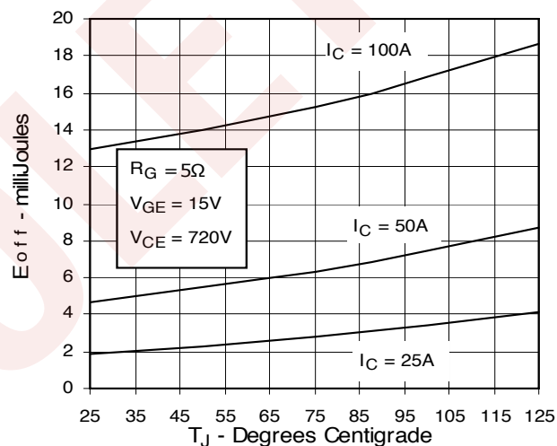
Fig. 10. Dependence of Turn-off Energy Loss on Temperature
