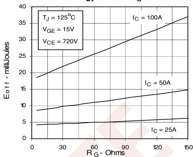
Fig. 8. Dependence of Turn-off Energy Loss on R_G
