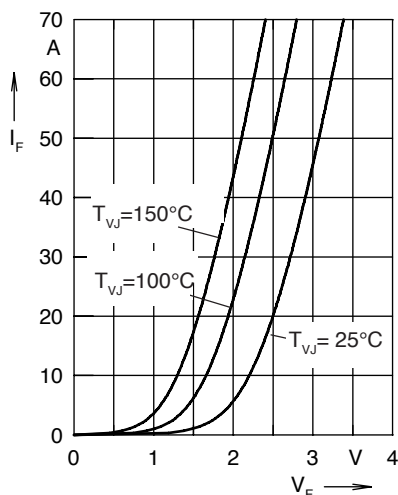
Fig. 18. Forward current I_F versus V_F
