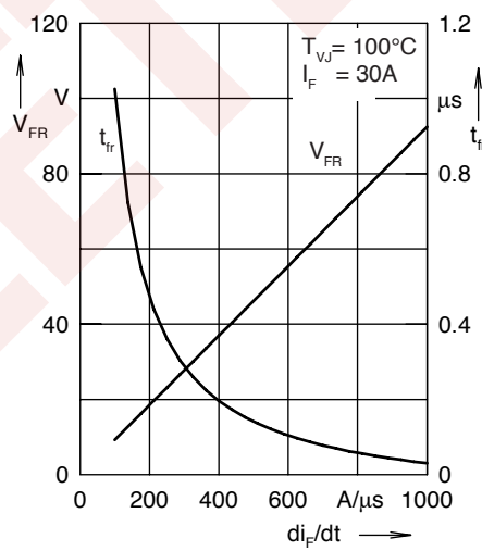
Fig. 23. Peak forward voltage V_{FR} and t_{fr} versus di_F/dt
