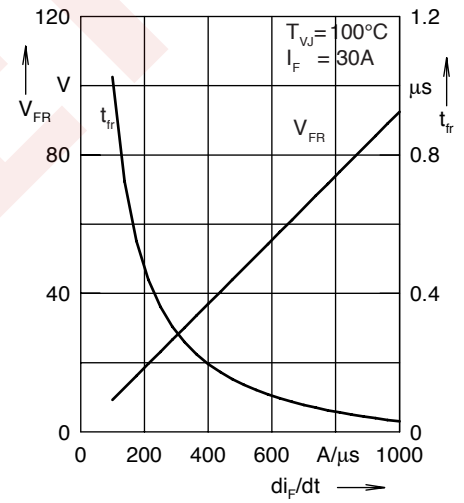
Fig. 29. Peak forward voltage V_{FR} and t_{fr} versus di_F/dt
