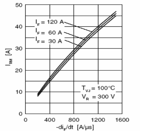
Fig. 23 Typ. peak reverse current I_{RM}
