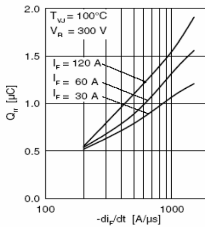
Fig. 22 Typ. Reverse Recovery Charge Q_{rr}
