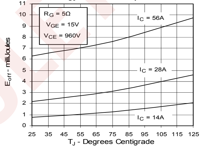
Fig. 10. Dependence of Turn-off Energy Loss on Temperature
