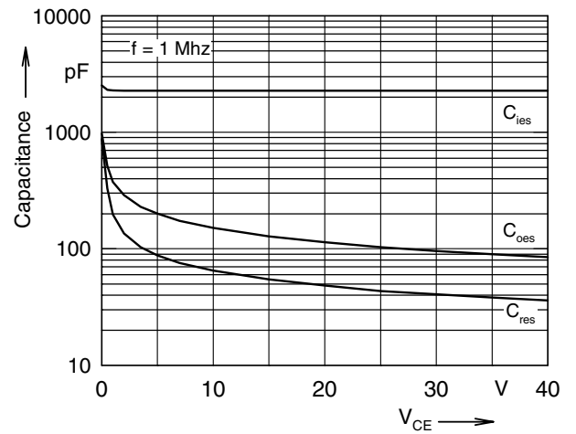
Fig. 4 Capacitance curves
