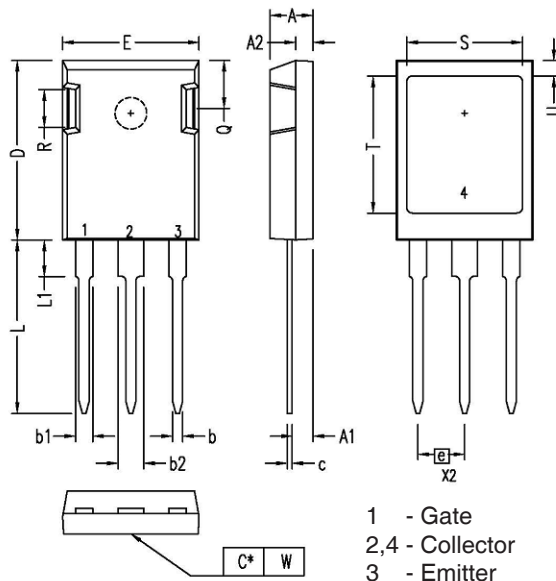
ISOPLUS247 (IXXR) Outline
