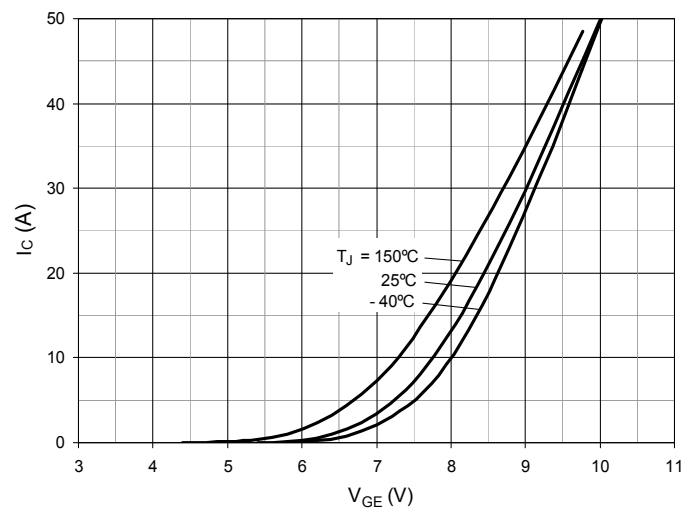
Fig. 6. Input Admittance
