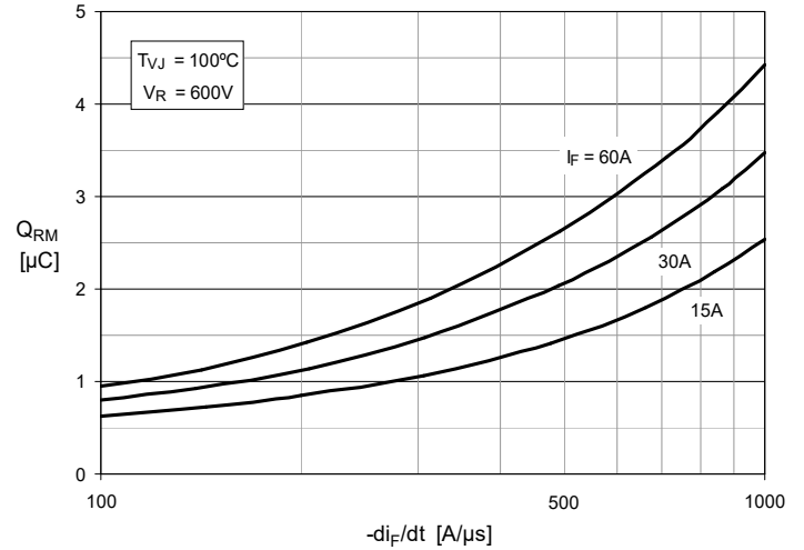
Fig. 24. Reverse Recovery Charge Q_{RM} vs. -di_F/dt
