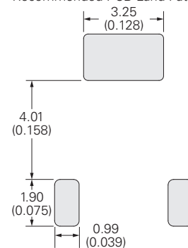
Recommended PCB Land Pattern
