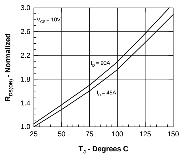
Fig.4 Temperature Dependence of Drain to Source Resistance
