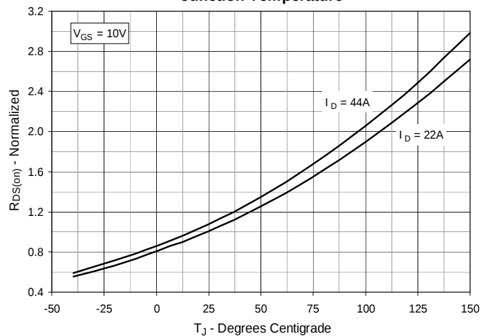
Fig. 4. R_{DS(on)} Normalized to I_D = 22A Value vs. Junction Temperature
