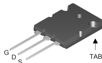
TO-264 (IXFK)
