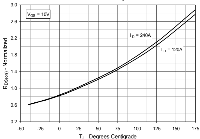
Fig. 4. R_{DS(on)} Normalized to I_D = 120A Value vs. Junction Temperature
