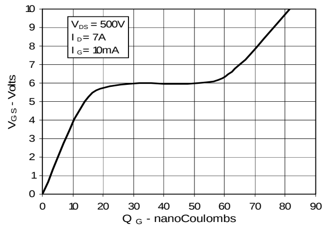
Fig. 10. Gate Charge
