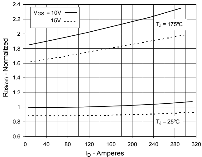
Fig. 5. R_{DS(on)} Normalized to I_D = 91\text{A} Value vs. Drain Current
