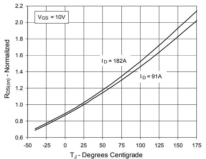
Fig. 4. R_{DS(on)} Normalized to I_D = 91\text{A} Value vs. Junction Temperature
