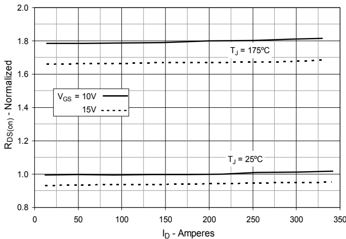
Fig. 5. R_{DS(on)} Normalized to I_D = 210A Value vs. Drain Current
