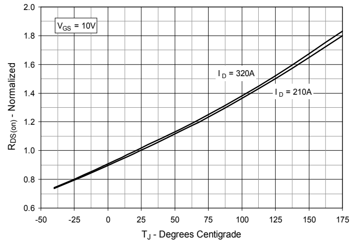
Fig. 4. R_{DS(on)} Normalized to I_D = 210A Value vs. Junction Temperature
