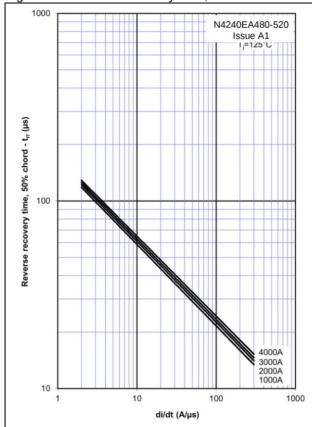
Figure 8 – Reverse recovery time, t_{rr}
