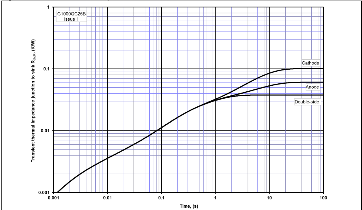
Figure 4 – Transient thermal impedance
