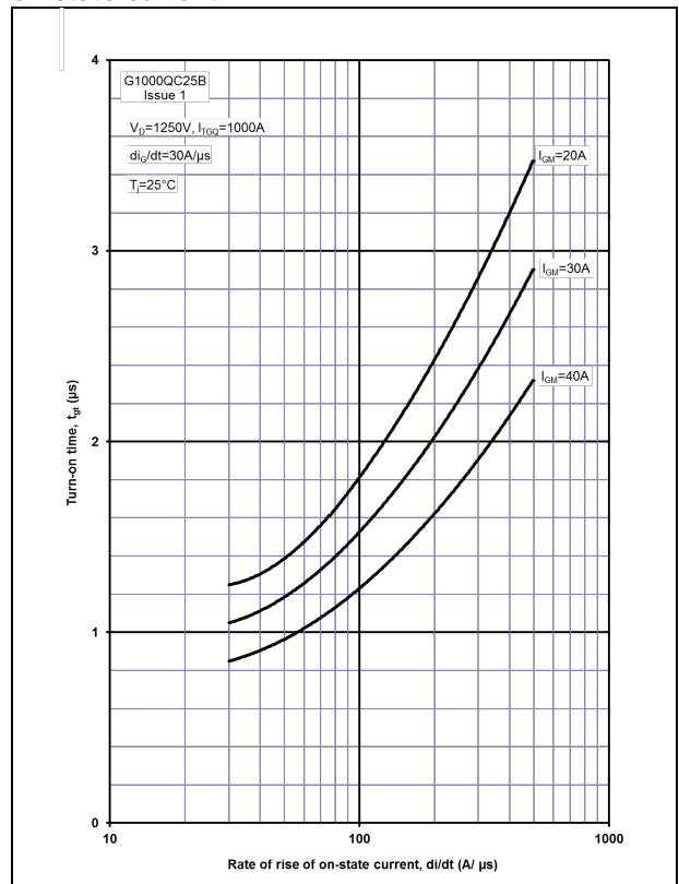
Figure 8 – Typical turn-on time vs. rate of rise of on-state current
