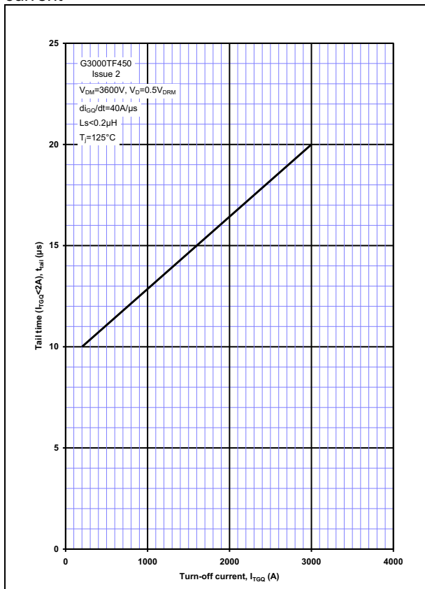
Figure 15 – typical tail time ( I_{TGO}<2\text{A} ) vs. turn-off current
