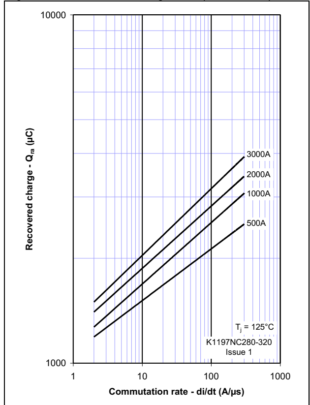
Figure 6 - Recovered charge, Q_{ra} (50% chord) (μC)
