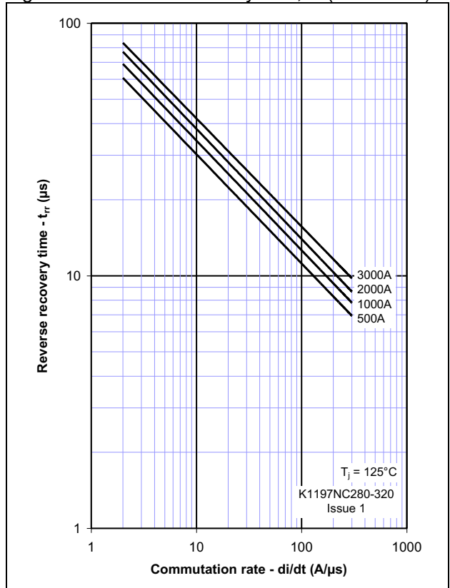
Figure 8 - Maximum recovery time, t_{rr} (50% chord) (μs)
