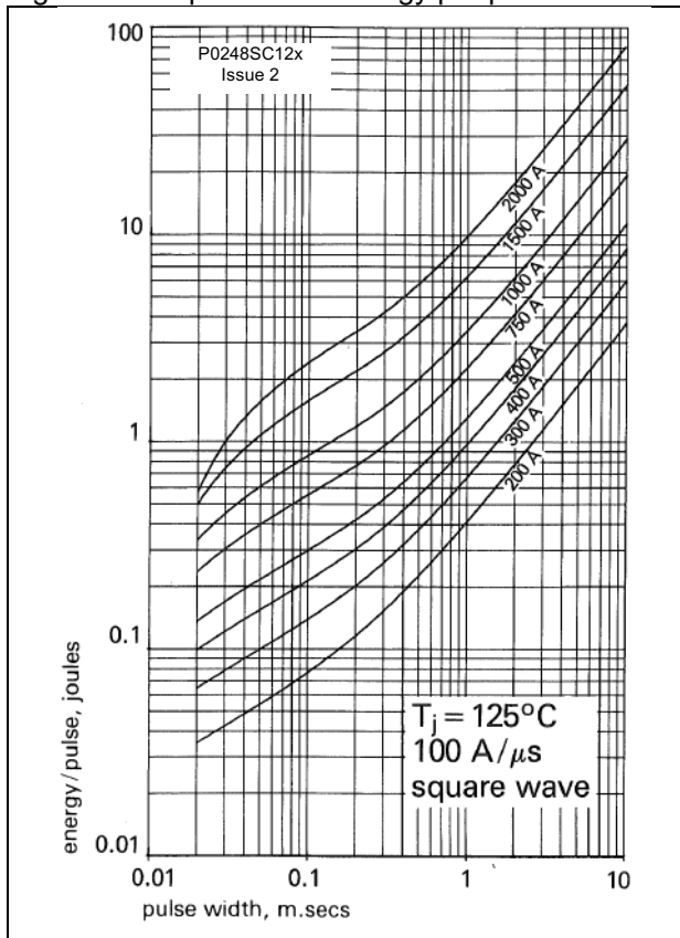
Figure 13 - Square wave energy per pulse
