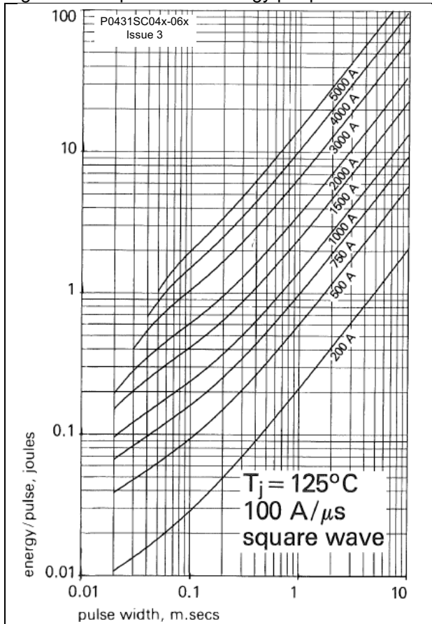
Figure 13 - Square wave energy per pulse
