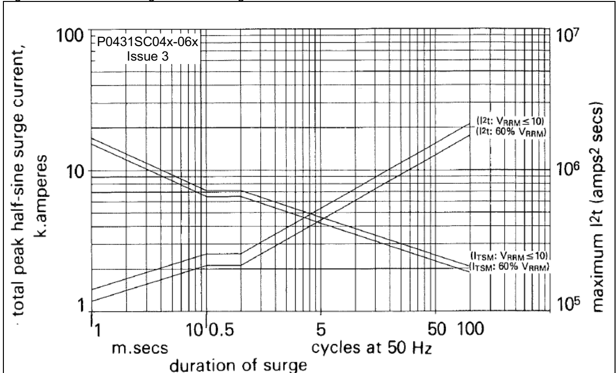
Figure 15 - Maximum surge and I^2t Ratings
