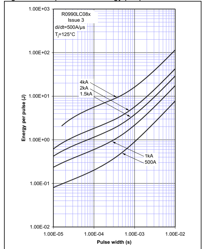
Figure 18 - Square wave energy per pulse
