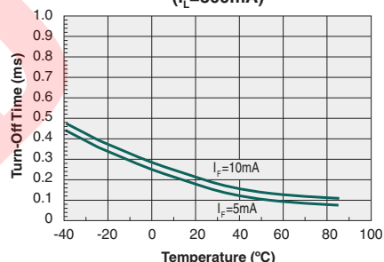
Typical Turn-Off Time vs. Temperature ( I_L = 300\text{mA} )
