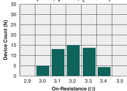
Typical On-Resistance Distribution (N=50, I_F=2\text{mA} , I_L=300\text{mA} )
