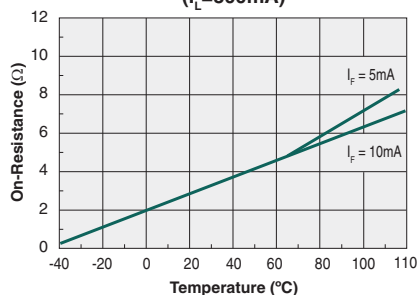
Typical On-Resistance vs. Temperature ( I_L = 300\text{mA} )
