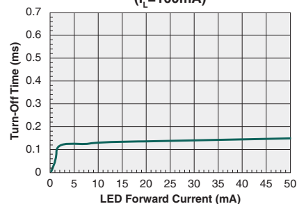
Turn-Off Time vs. LED Forward Current ( I_L = 100\text{mA} )
