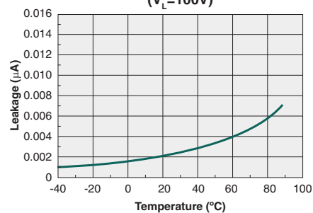
Typical Leakage vs. Temperature Measured Across Pins 3 & 4 ( V_L = 100\text{V} )
