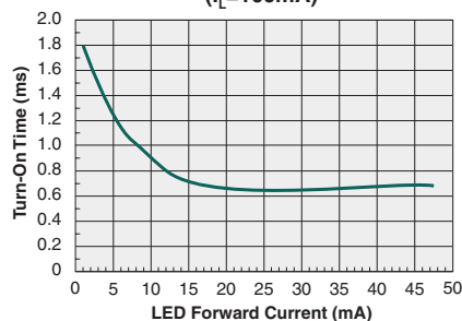
Turn-On Time vs. LED Forward Current ( I_L = 100\text{mA} )
