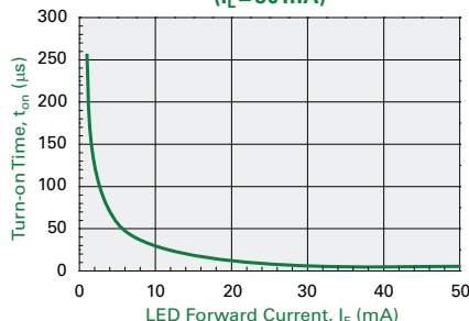
Typical Turn-on Time vs. LED Forward Current ( I_L = 50 mA)
