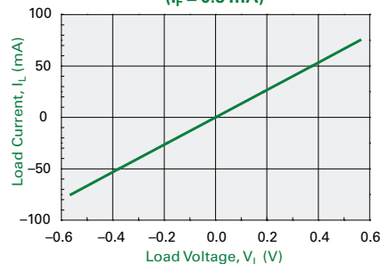
Typical Load Current vs. Load Voltage ( I_F = 0.5 mA)
