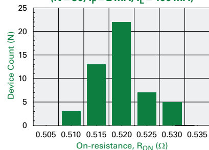
Typical On-resistance Distribution (N = 50, I_F = 2 mA, I_L = 400 mA)
