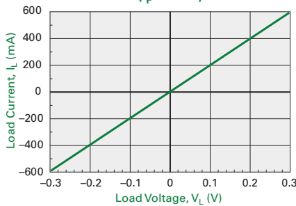
Typical Load Current vs. Load Voltage ( I_F = 1 mA)
