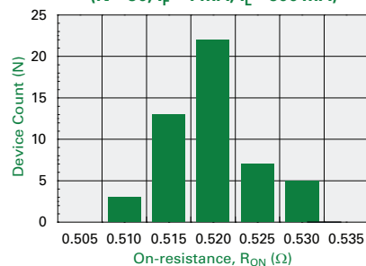
Typical On-resistance Distribution (N = 50, I_F = 1 mA, I_L = 600 mA)
