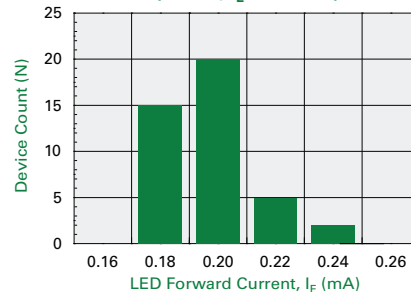
Typical I_F for Switch Dropout (N = 50, I_L = 600 mA)
