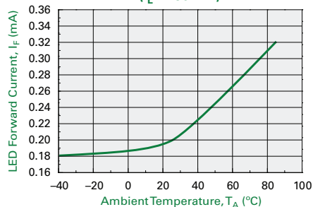
Typical I_F for Switch Dropout vs. Temperature ( I_L = 480 mA)
