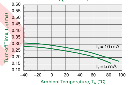
Typical Turn-off Time vs. Temperature ( I_L = 80 mA)
