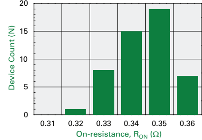
Typical On-resistance Distribution (N = 50, I_F = 2 mA, I_L = 0.75 A)
