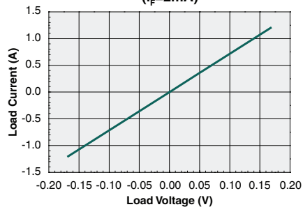
Typical Load Voltage vs. Load Current ( I_F=2\text{mA} )
