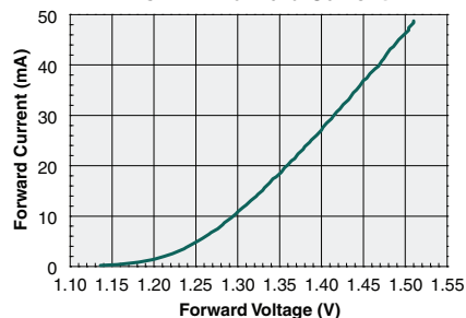
LED Forward Voltage vs. LED Forward Current
