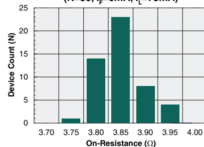
Typical On-Resistance Distribution (N=50, I_F=0\text{mA} , I_L=75\text{mA} )
