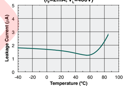
Leakage Current vs. Temperature Measured Across Pins 3 & 4 (I_F=2\text{mA}, V_L=400\text{V})
