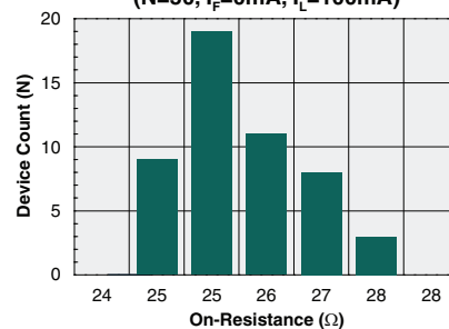
Typical On-Resistance Distribution (N=50, I_F=0\text{mA} , I_L=100\text{mA} )
