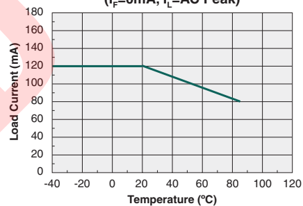
Maximum Load Current vs. Temperature ( I_F=0\text{mA} , I_L=\text{AC Peak} )
