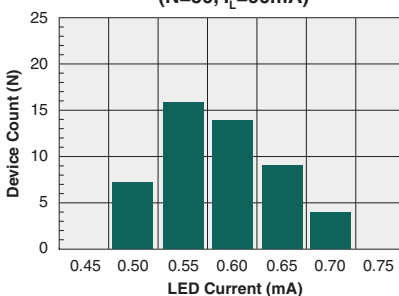
Typical I_F for Switch Operation (N=50, I_L=90\text{mA} )
