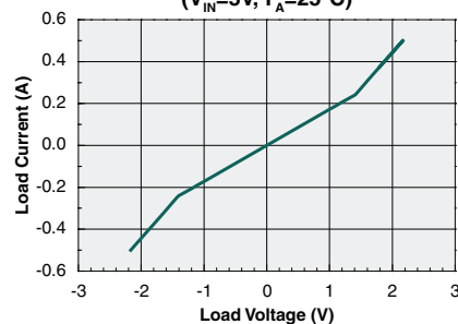
Typical Load Current vs. Load Voltage ( V_{IN}=5V, T_A=25^\circ C )
