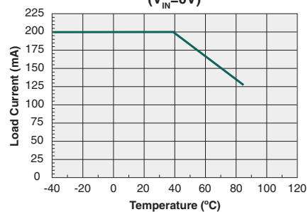
Typical Maximum Load Current vs. Temperature ( V_{IN}=0V )
