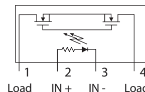
CPC1219Y Pinout
