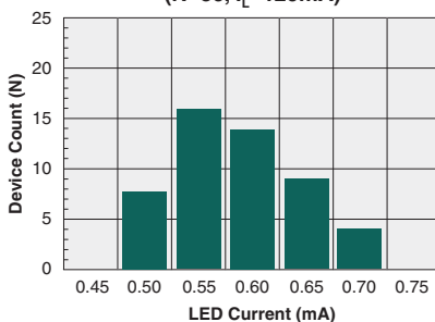
Typical I_F For Switch Operation (N=50, I_L=120\text{mA} )
