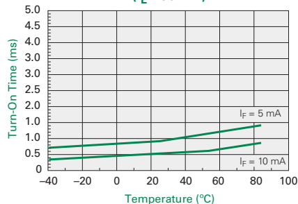
Typical Turn-On Time vs. Temperature ( I_L = 80 \text{ mA} )
