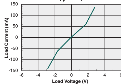
Typical Load Current vs. Load Voltage ( I_F=0\text{mA} )
