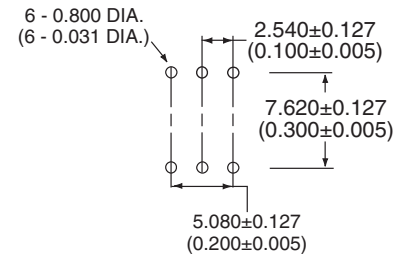
PCB Hole Pattern
