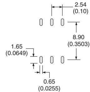
PCB Land Pattern
