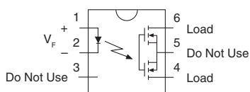
AC/DC Configuration
