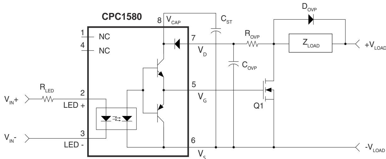
Figure 3. CPC1580 Over-Voltage Protection for Inductive Loads
