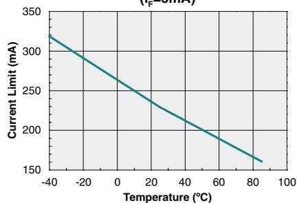
AC/DC Configuration Current Limit vs. Temperature ( I_F=5\text{mA} )
