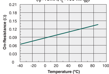
Typical On-Resistance vs. Temperature
