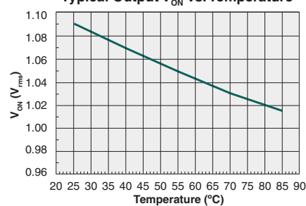
Typical Output V_{\text{ON}} vs. Temperature
