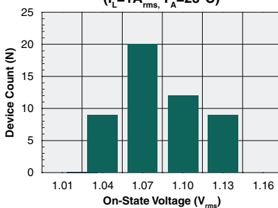
Typical On-State Voltage (I_L=1\text{A}_{\text{rms}}, T_A=25^\circ\text{C})
