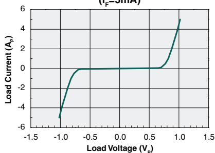
Typical Load Voltage vs. Load Current ( I_F=5\text{mA} )
